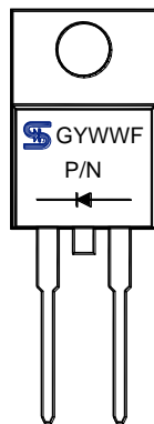
MARKING DIAGRAM
