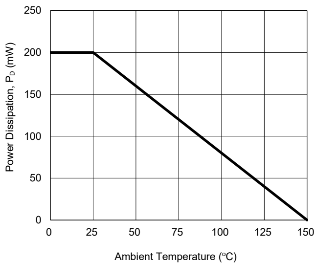
Fig.2 Derating Curve
