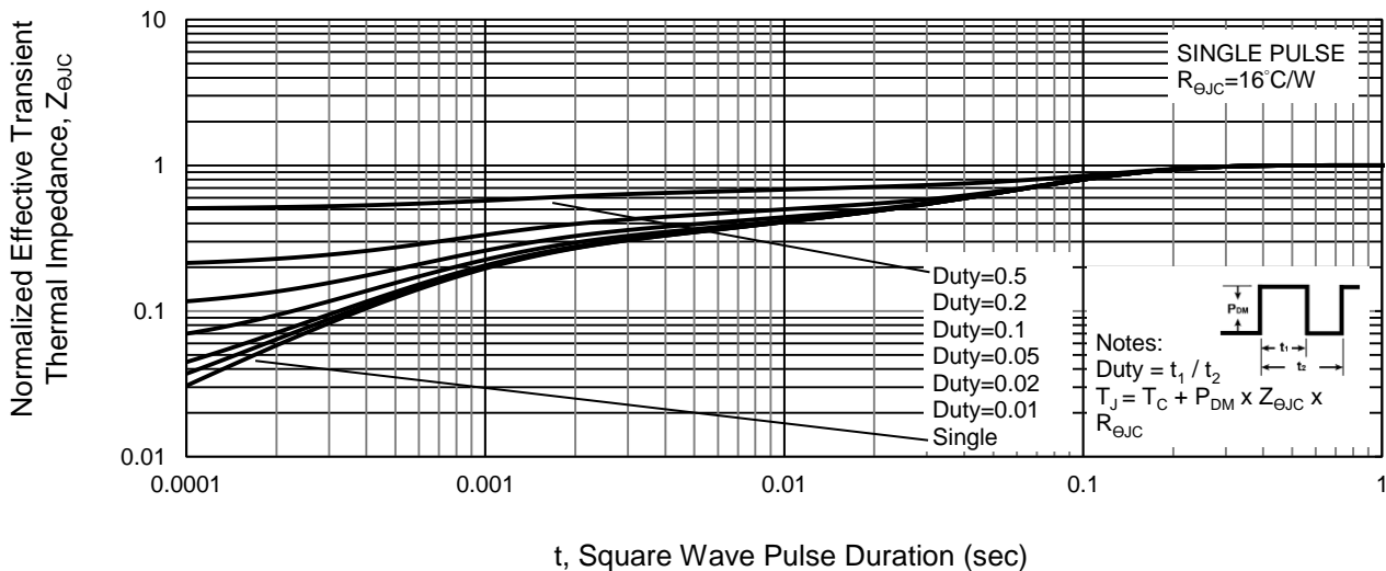
Normalized Thermal Transient Impedance, Junction-to-Cas
