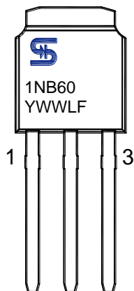
MARKING DIAGRAM
