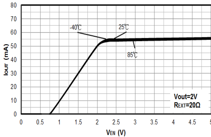
Figure 15. V_{EN} vs. I_{OUT} ( R_{EXT}=20\Omega )
