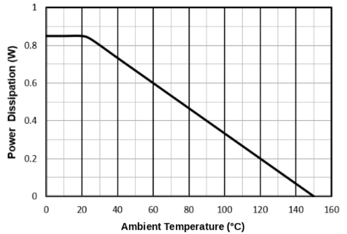
Figure 10. P_D vs. Ambient Temperature
