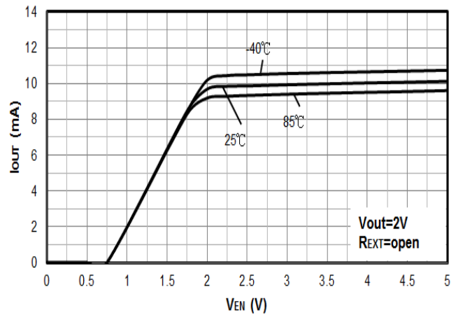
Figure 14. V_{EN} vs. I_{OUT} ( R_{EXT}=open )
