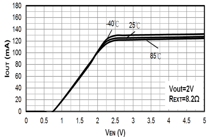
Figure 16. V_{EN} vs. I_{OUT} ( R_{EXT}=8.2\Omega )
