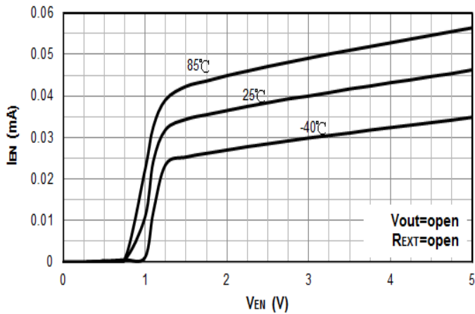
Figure 17. V_{EN} vs. I_{EN} ( R_{EXT}=open )
