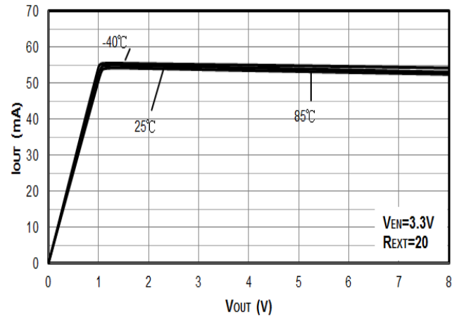
Figure 12. V_{OUT} vs. I_{OUT} ( R_{EXT}=20\Omega )
