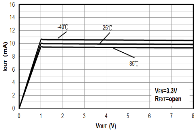
Figure 11. V_{OUT} vs. I_{OUT} ( R_{EXT}=open )
