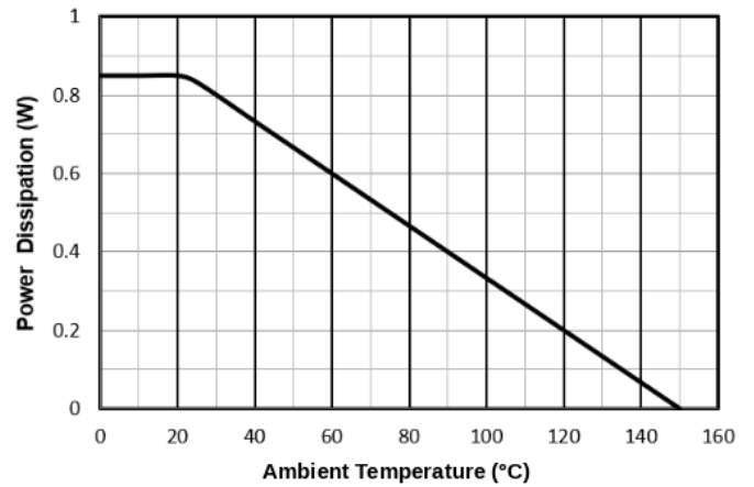
Figure 20. P_D vs. Ambient Temperature
