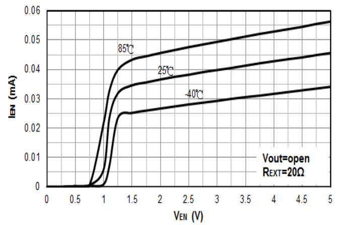
Figure 18. V_{EN} vs. I_{EN} ( R_{EXT}=20\Omega )
