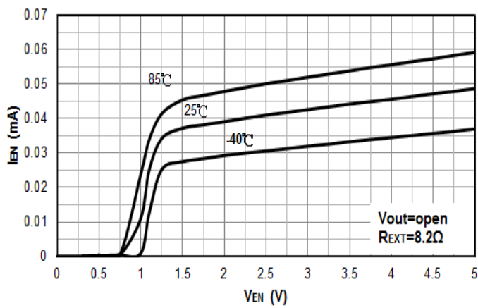
Figure 19. V_{EN} vs. I_{EN} ( R_{EXT}=8.2\Omega )
