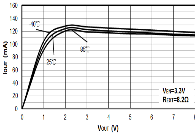
Figure 13. V_{OUT} vs. I_{OUT} ( R_{EXT}=8.2\Omega )
