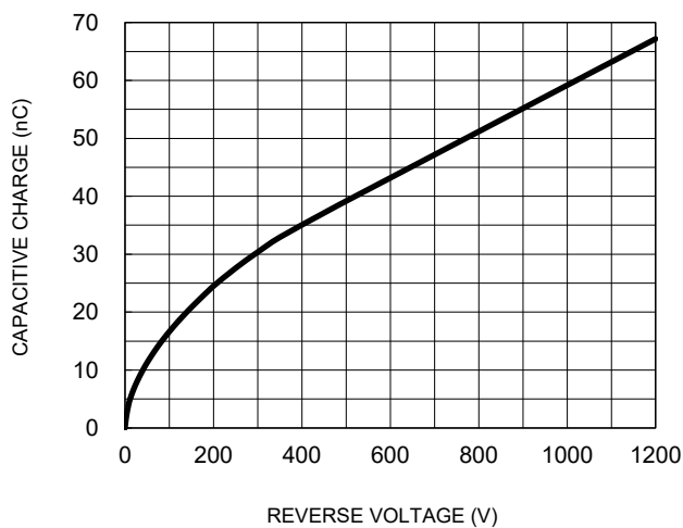
Fig.5 Typical Capacitive Charge
