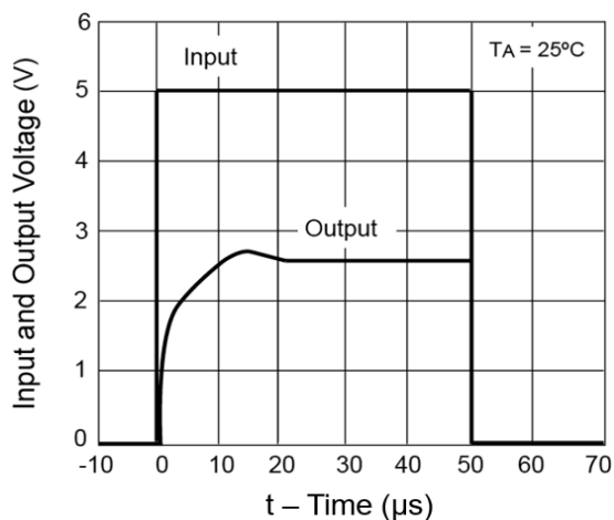
Figure 14. Pulse Response
