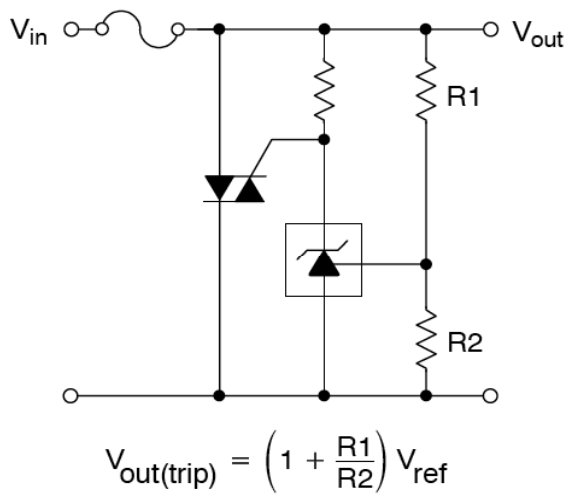
Figure 7. TRIAC Crowbar
