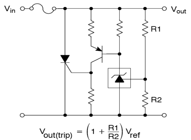
Figure 8. SCR Crowbar
