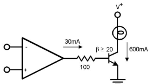
Figure 2. Lamp Driver
