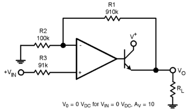
Figure 6. Power Amplifier
