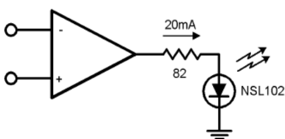
Figure 1. LED Driver
