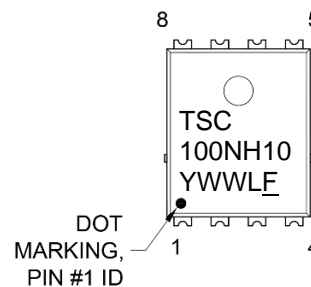
MARKING DIAGRAM
