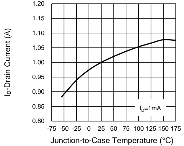
Drain Current
