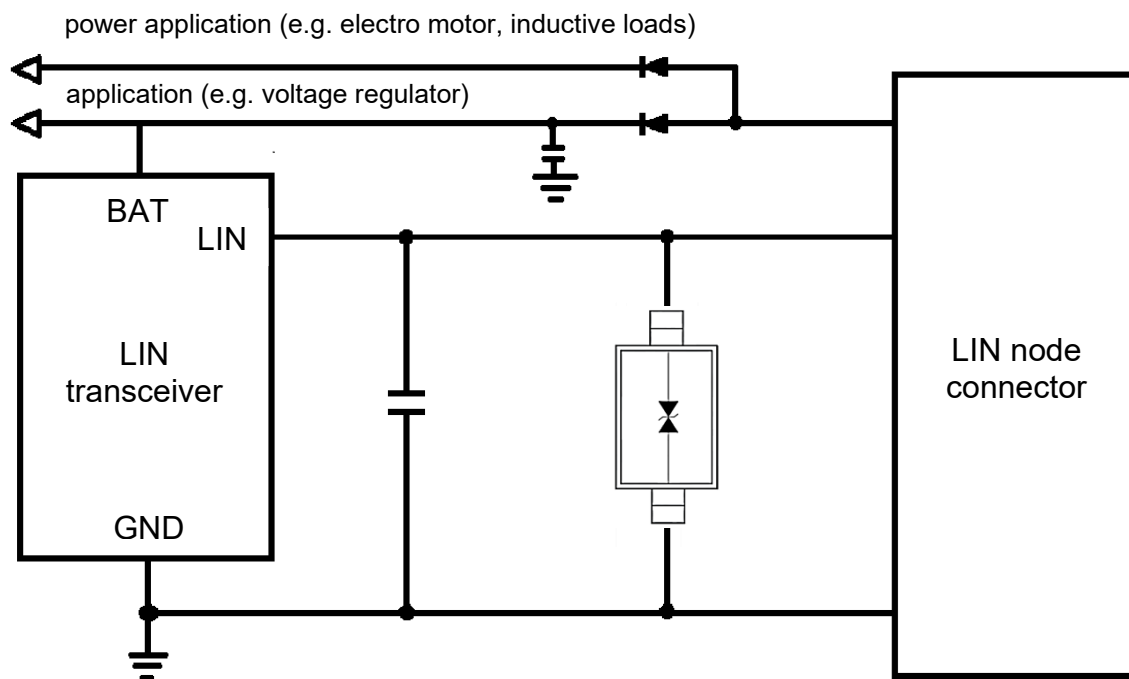
Fig.1 ESD protection by TESDA27VB17P1M3
