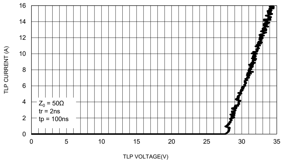
Fig.5 TLP Curve
