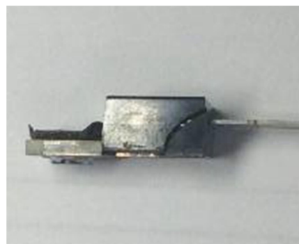
(b) Mold compound crack
