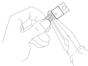
(a) Correct method
