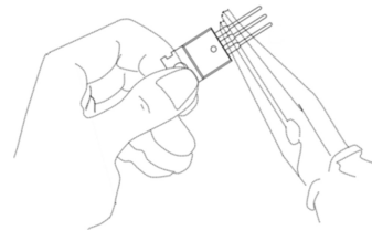
(b) wrong method
