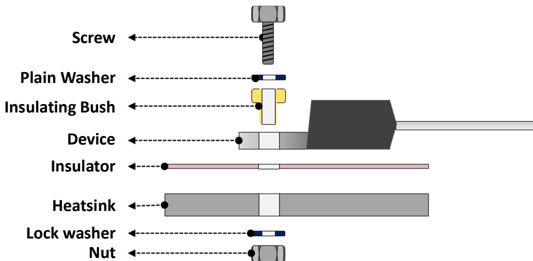
Fig 6. Screw mounting of TO-220
