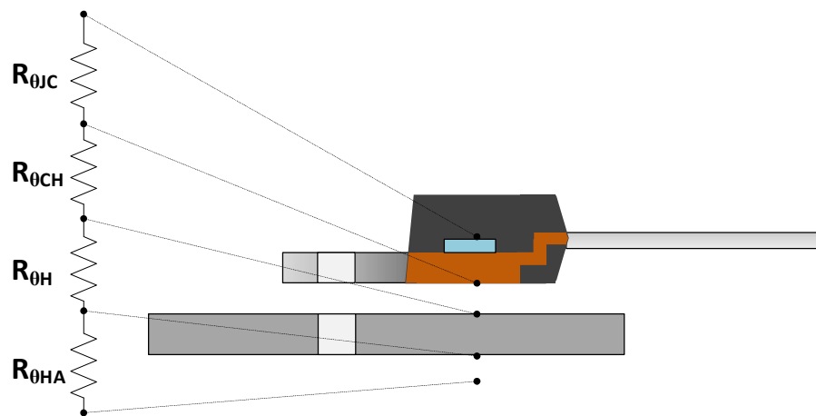
Fig 1. Thermal resistance structure
