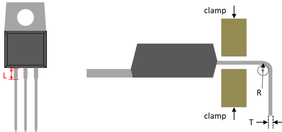
Fig 8. Lead forming and cutting
