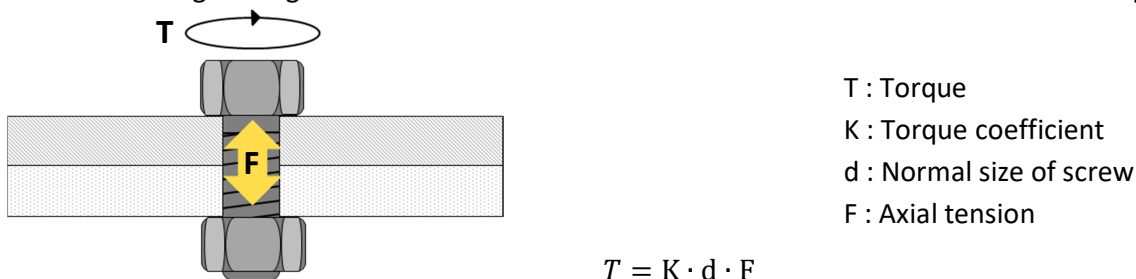
Fig 5. The relationship between torque and axial tension
