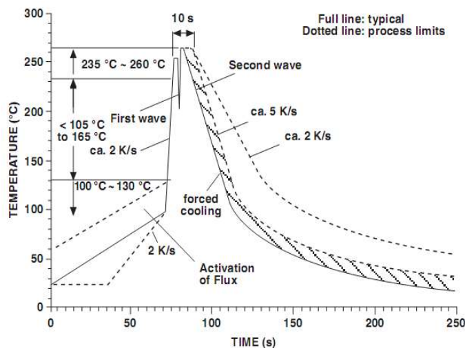
Fig.10 Dual wave Solder profile
